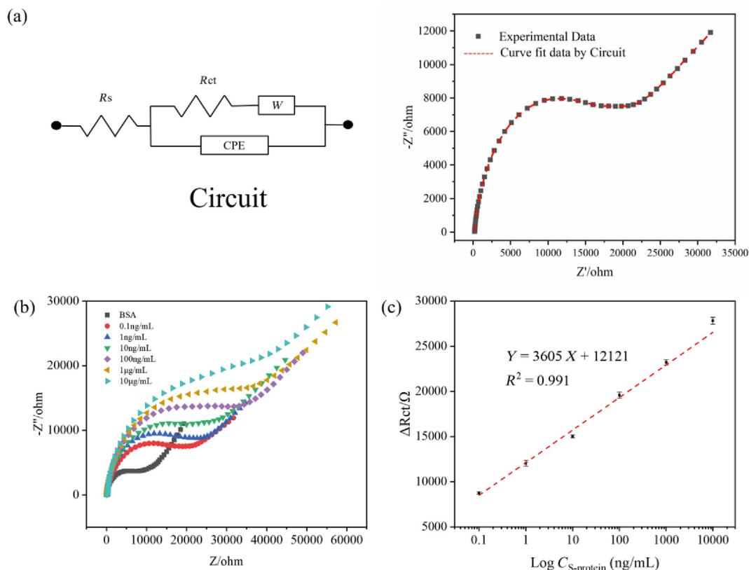
Fig. 7. (a) The modified Randles circuit with CPE element. R_s solution resistant; CPE, constant phase element; R_{ct} , charge transfer resistant; W , Warburg resistant. (b) Nyquist plots obtained \text{Fe}_3\text{O}_4/\text{SiO}_2\text{-Au/GCE} at various concentrations of SARS-CoV-2 S-protein and (c) the plot of logarithm concentrations against \Delta R_{ct} .
