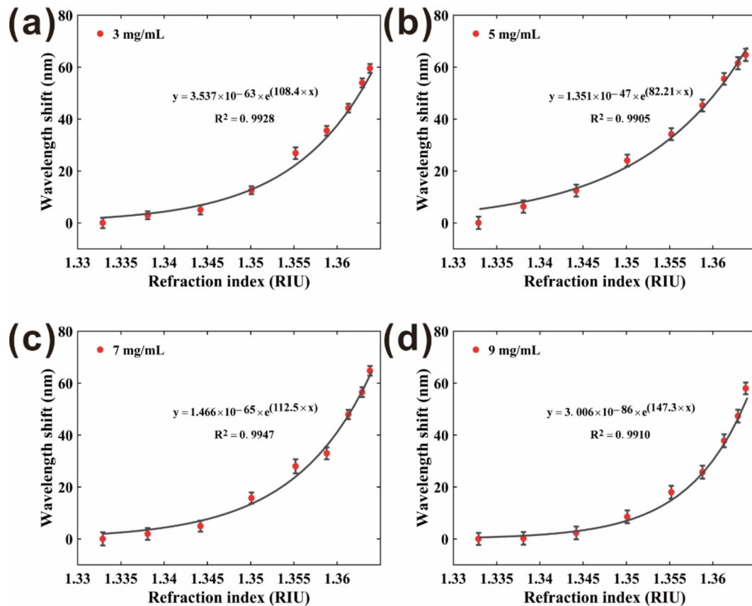
Fig. 4. Fitting curves of relationship between resonance wavelength shift (compared with RI:1.3329) of sensors fabricated by DA concentration of (a) 3, (b) 5, (c) 7 and (d) 9 mg/mL and refractive index.
