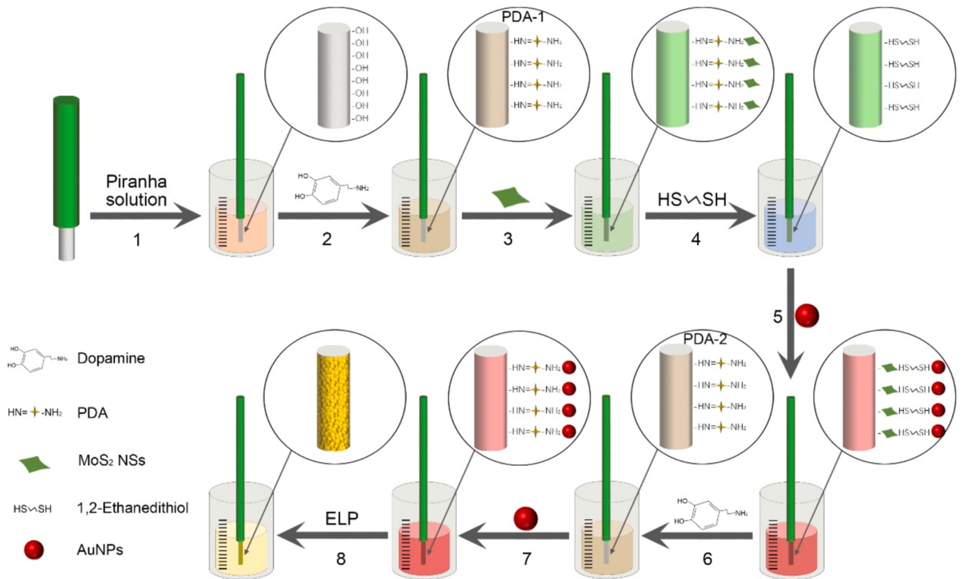
Fig. 1. Schematic illustration of the ELP fabrication of optical fiber sensor with fiber/MoS 2 /AuNPs/Au structure.
