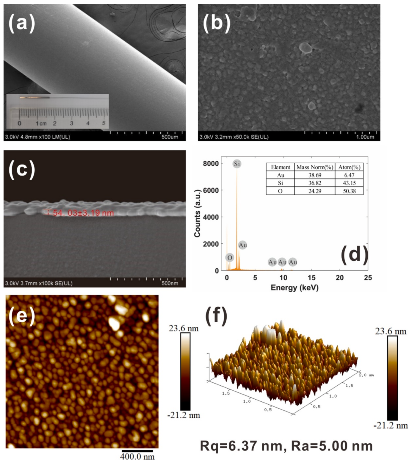
Fig. 5. SEM images of (a) top view, (b) surface morphology, (c) cross section of electroless-plated Au film coated optical fiber probe with fiber/Au structure. The inset in (a) is the photograph of the optical fiber SPR sensor. (d) The EDS spectrum of optical fiber probe with fiber/Au structure. (e, f) AFM images of electroless-plated Au film. Two profile roughness parameters, including roughness average (Ra), RMS roughness (Rq), were labeled at the bottom.
