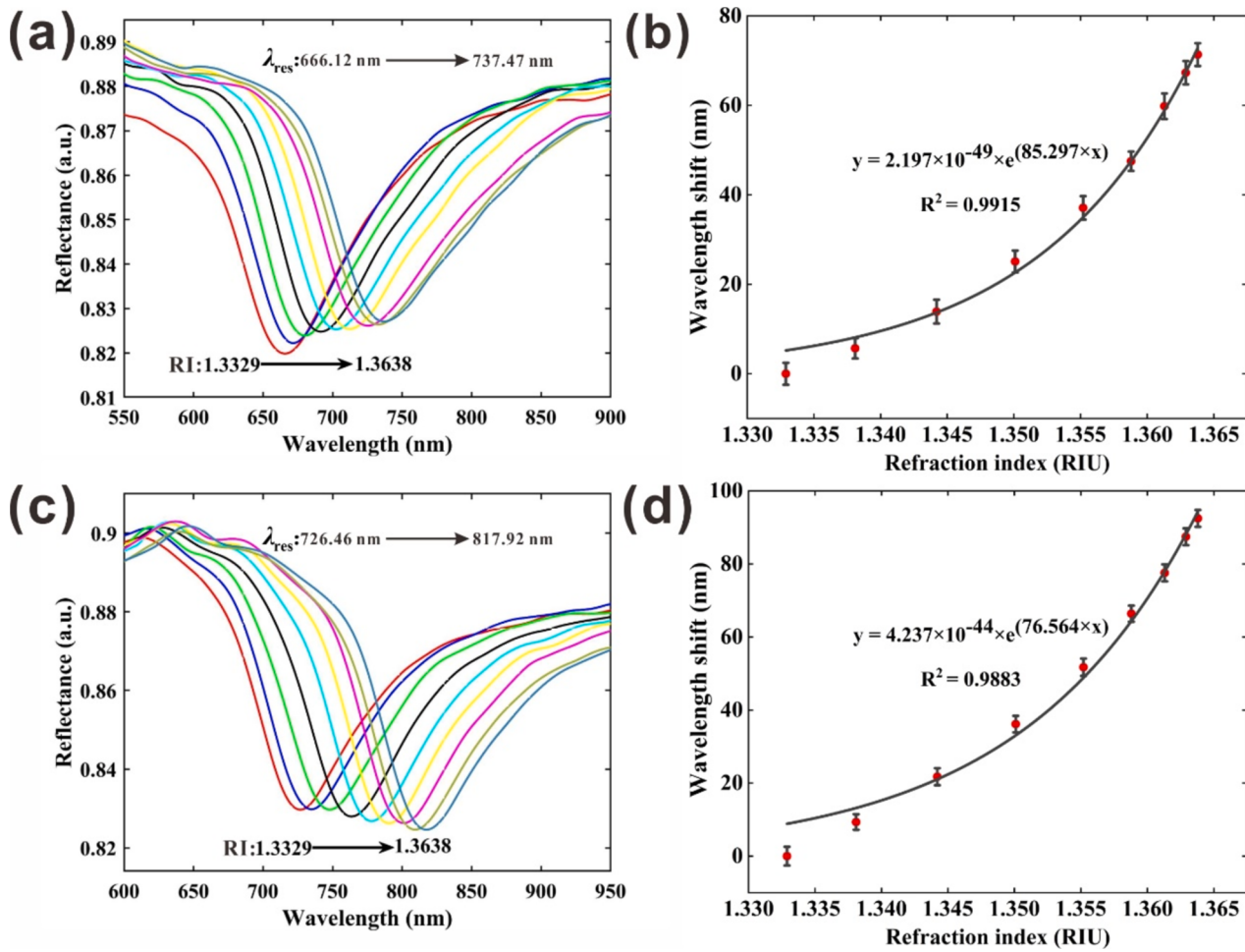
Fig. 8. Spectra of optical fiber SPR sensor with fiber/Au structure in solvents with different RI values (a) and refractive index sensitivity fitting curve (b). Spectra of optical fiber SPR sensor with fiber/MoS 2 /AuNPs/Au structure in solvents with different RI values (c) and refractive index sensitivity fitting curve (d).
