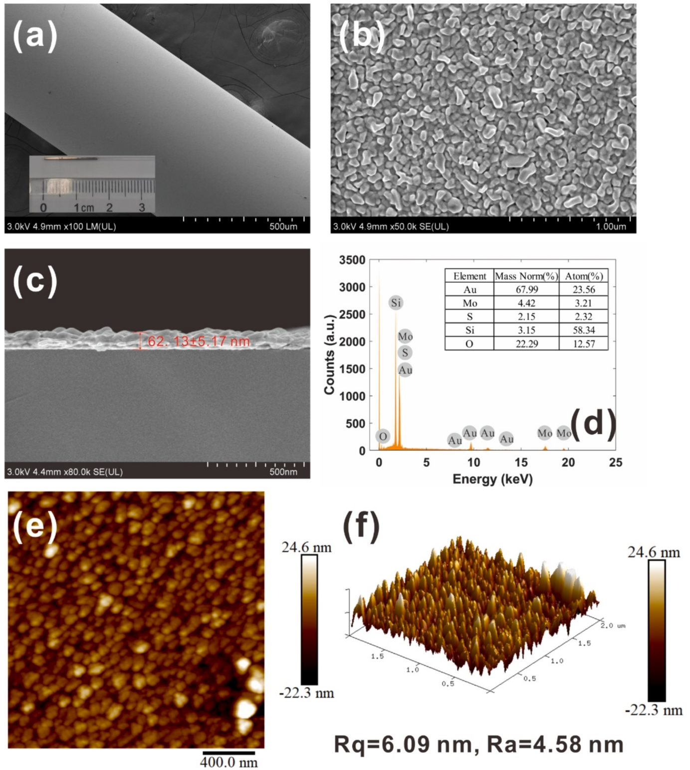
Fig. 7. SEM images of (a) top view, (b) surface morphology, (c) cross section of electroless-plated Au film coated optical fiber probe with fiber/MoS 2 /AuNPs/Au structure. The inset in (a) is the photograph of the optical fiber SPR sensor. (d) The EDS spectrum of optical fiber probe with fiber/MoS 2 /AuNPs/Au structure. (e, f) AFM images of electroless-plated Au film. Two profile roughness parameters, including roughness average (Ra), RMS roughness (Rq), were labeled at the bottom.
