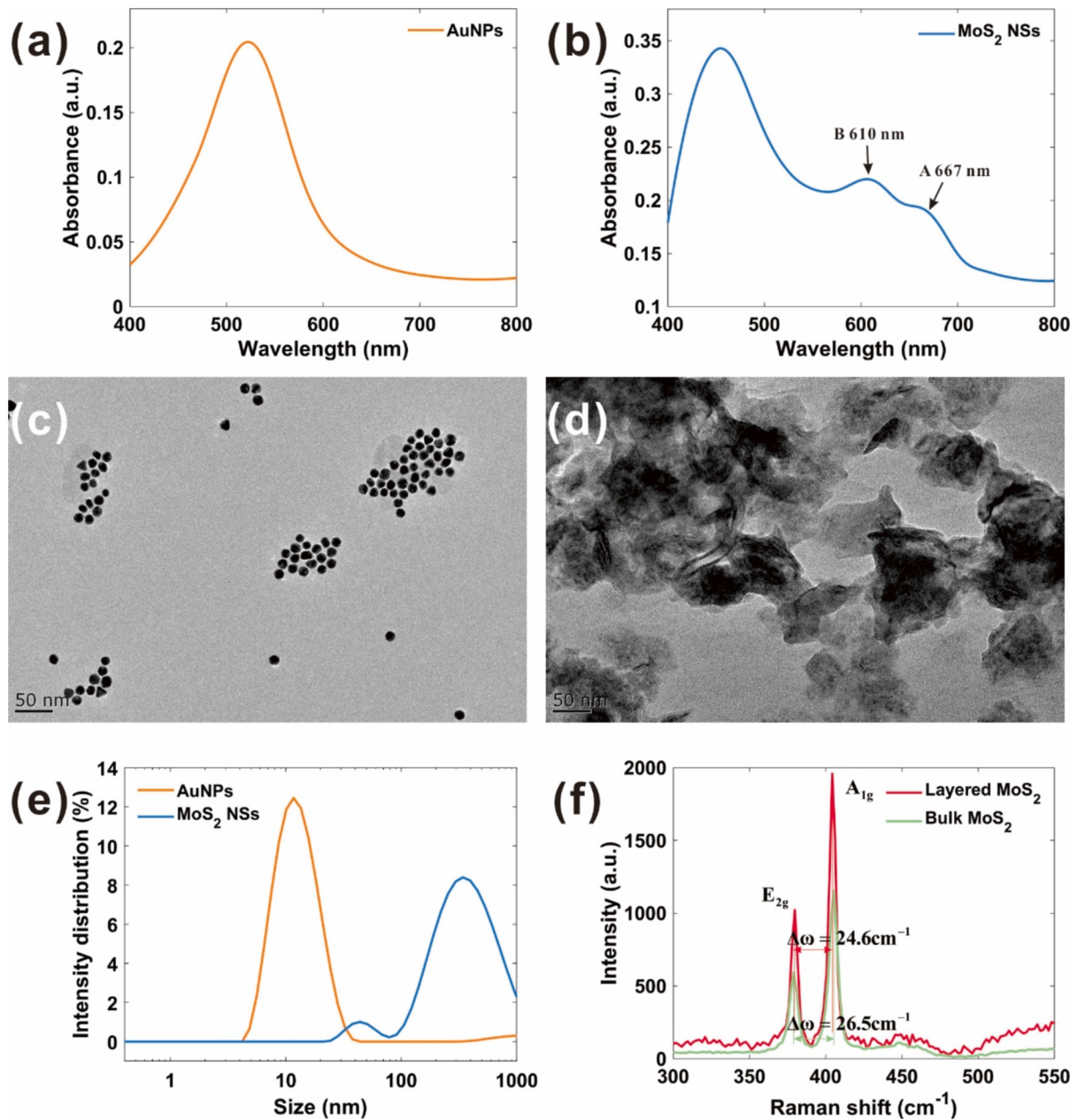
Fig. 2. Absorption spectra of (a) AuNPs and (b) layered MoS 2 NSs. TEM micrographs of (c) AuNPs and (d) MoS 2 NSs. (e) DLS spectra of AuNPs and MoS 2 NSs. (f) Raman spectra of bulk MoS 2 and MoS 2 NSs.
