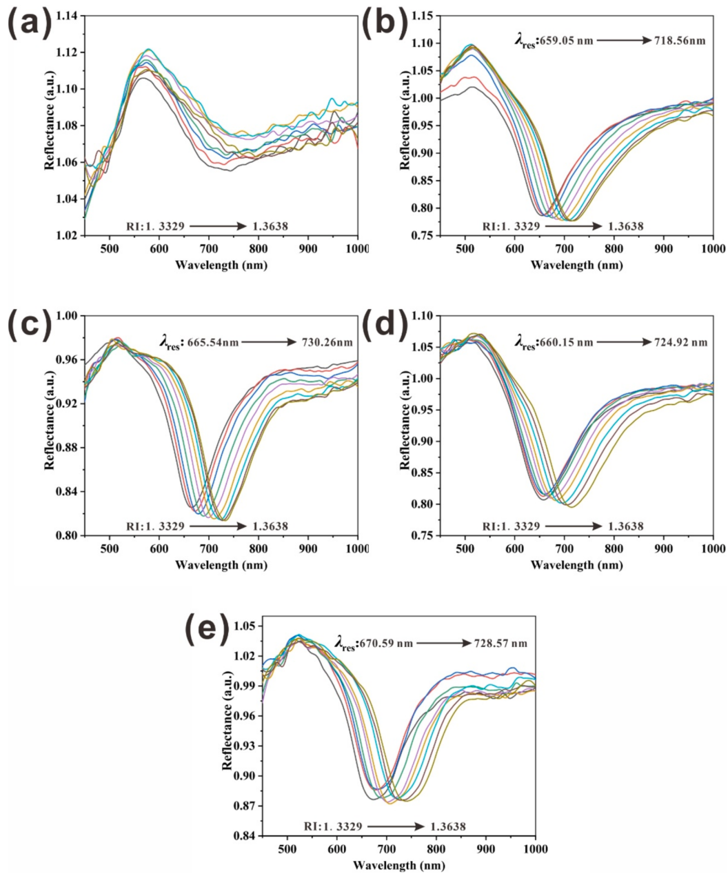
Fig. 3. Reflection spectra of optical fibers with fiber/Au structure fabricated by DA concentration of (a) 1, (b) 3, (c) 5, (d) 7 and (e) 9 mg/mL in solvents with different refractive index (RI) values.
