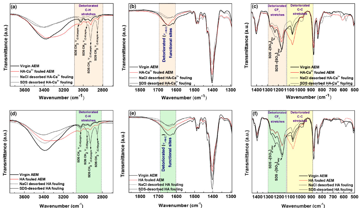
Fig. 5. ATR-FTIR spectra of 2% (w/w) NaCl and 0.03% (w/w) SDS desorbed fouled membranes. (a) High ( \nu , 4000–2500 \text{cm}^{-1} ), (b) mid ( \nu , 1800–1300 \text{cm}^{-1} ) and (c) low ( \nu , 1400–500 \text{cm}^{-1} ) frequency spectral regions of HA- \text{Ca}^{2+} fouled membranes. (d) High ( \nu , 4000–2500 \text{cm}^{-1} ), (e) mid ( \nu , 1800–1300 \text{cm}^{-1} ) and (f) low ( \nu , 1400–500 \text{cm}^{-1} ) frequency spectral regions of HA fouled membranes.
