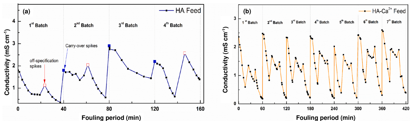
Fig. 1. Conductivity (mS cm –1 ) vs fouling period (min) plot of feed solutions containing (a) Sigma-Aldrich humic acid (~2 mg L –1 , TOC), 0.001 M NaCl and 0.001 M NaHCO 3 at pH ~8 (HA) and (b) Sigma-Aldrich humic acid (~2 mg L –1 , TOC), 0.001 M NaCl, 0.001 M NaHCO 3 and CaCl 2 ·2H 2 O (~200 mg L –1 , Ca 2+ ) at pH ~8 (HA-Ca 2+ )
