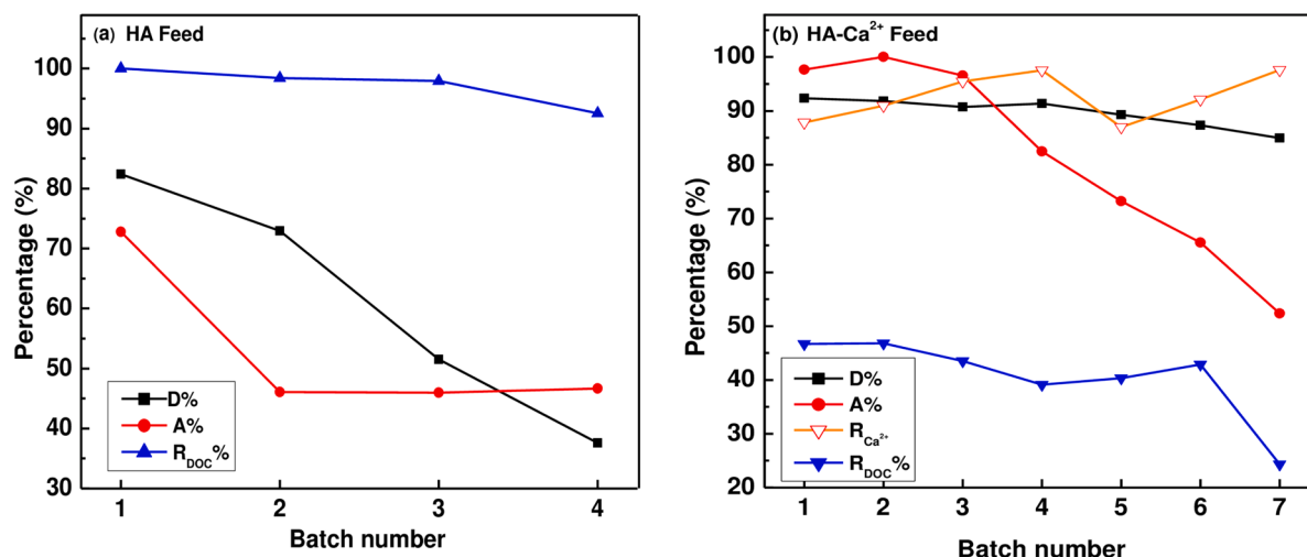
Fig. 2. Variation of desalination (D%), decolourisation (A%) and removal of DOC and/or \text{Ca}^{2+} ( R_{\text{DOC}}\% ) ( R_{\text{Ca}^{2+}}\% ) as a function of feed solution cycles in the presence of HA ( \sim 2 \text{ mg L}^{-1} , TOC, 0.001 M NaCl and 0.001 M \text{NaHCO}_3 at pH \sim 8 ) or HA- \text{Ca}^{2+} ( \sim 2 \text{ mg L}^{-1} , TOC, 0.001 M NaCl, 0.001 M \text{NaHCO}_3 and \sim 200 \text{ mg L}^{-1} , \text{Ca}^{2+} at pH \sim 8 )
