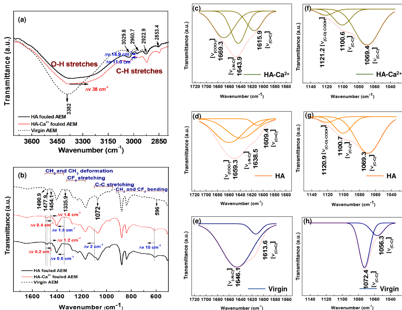
Fig. 4. FTIR-ATR spectra of virgin, HA fouled and HA-Ca 2+ fouled CJMA-4 AEMs at (a) high frequency ( \nu , 4000–2500 cm -1 ) and (b) low frequency ( \nu , 1800–400 cm -1 ) spectral regions with O–H stretching ( \nu , 3670–3070 cm -1 ), C–H stretching ( \nu , 3070–2800 cm -1 ), C=C stretching ( \nu , 1750–1550 cm -1 ), CH 2 and CH 3 deformations ( \nu , 1515–1145 cm -1 ), C–C stretching ( \nu , 1090–900 cm -1 ) and CH 2 bending ( \nu , >800 cm -1 ) vibrations to illustrate peak shifts due to membrane-foulant interactions. (c–e) De-convoluted spectral regions illustrating foulant features of HA-Ca 2+ , HA fouled membranes and virgin membrane for the range 1720–1660 cm -1 . (f–h) De-convoluted spectral regions illustrating foulant features of HA-Ca 2+ , HA fouled membranes and virgin membrane for the range 1140–1040 cm -1 .
