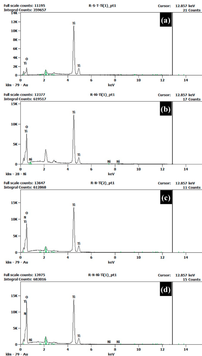
Fig. 2. EDX spectroscopy images of (a) un-doped (b) Ni-doped (c) N-doped and (d) Ni/N co-doped \text{TiO}_2 nanoparticles.
