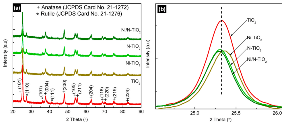
Fig. 1. (a) XRD patterns, and (b) expanded dominant anatase peak of un-doped, Ni-doped, N-doped and Ni/N co-doped TiO 2 nanoparticles.
