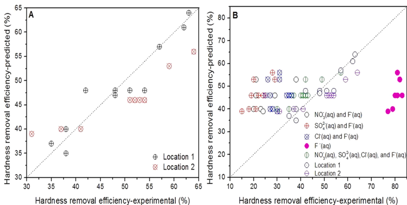
Fig. 1. Variations of hardness removal efficiency in A. groundwater of locations 1 and 2; symbols represent observations. Source water composition, current density and response time were related to Table 1 and 2. B. Simulated water by EC. Symbols represent various simulated water types. Model calculations were carried out with an RMS model developed for natural groundwater.
