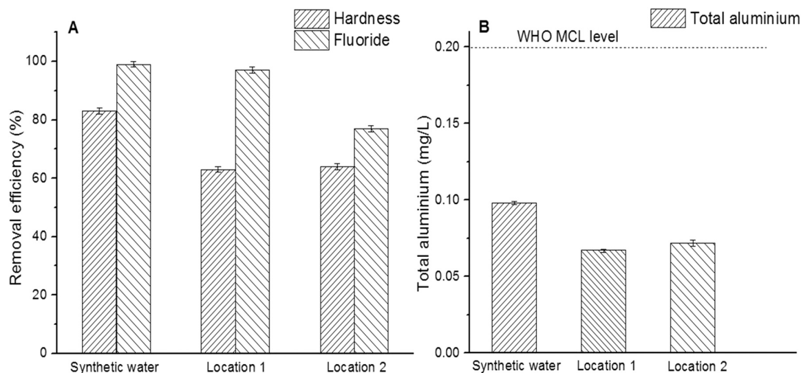
Fig. 3. A. Water hardness and fluoride removal efficiency using optimised EC. B. Residual aluminium concentration in treated water. Feed water composition is shown in Table 1 and Table 1-S. Vertical lines depict error bars.
