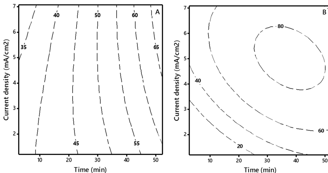
Fig. 2. Variation of hardness and fluoride removal efficiencies as a function of current density and process time. A. hardness B. fluoride as a function of time and current density for location 1. Source water composition: TDS 470 mg/L, hardness 183 mg/L \text{CaCO}_3 , fluoride 0.45 mg/L and pH 6.60.
