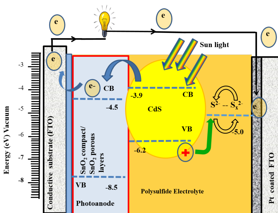
Figure 5: Energy band diagram of SnO 2 and working mechanism of CdS sensitized SnO 2 photoanode with compact SnO 2 layer.
