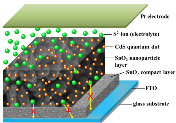
Figure 1: Schematic diagram showing the CdS sensitized solar cell with \text{SnO}_2 compact layer and porous nanoparticle (NP) \text{SnO}_2 layer.
