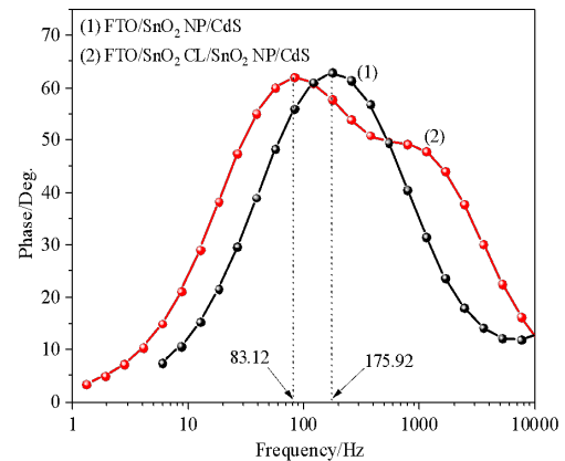
Figure 4: Bode phase plots of CdS QDSSCs (1) without and (2) with the SnO 2 compact layer in the photoanode, under the illumination of 100 mW cm -2 with AM 1.5 spectral filter.
