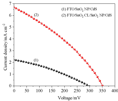
Figure 2: Current – voltage characterization of CdS QDSSCs (1) without and (2) with \text{SnO}_2 compact layer in the photoanode under the illumination of 100 \text{ mW cm}^{-2} .
