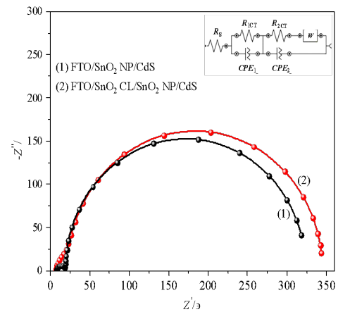
Figure 3: Nyquist plots of CdS QDSSCs (1) without and (2) with the \text{SnO}_2 compact layer in the photoanode, under the illumination of 100 \text{ mW cm}^{-2} with AM 1.5 spectral filter.
