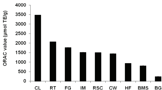
Fig. 1. ORAC values of various aqueous plant extracts - (CL) curry leaves, (RT) rooibos tea, (FG) fenugreek, (IM) Indian malabar, (RSC) red silk cotton tree, (CW) cowitch, (HF) holy fruit tree, (BMS) black mustard seed and (BG) bittergourd.
