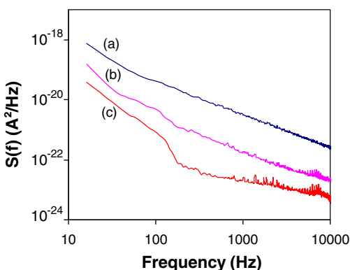
Fig. 4. Noise spectra of a nanocrystalline film of \text{ZnO} : (a) in air at a relative humidity of 70%; (b) in vacuum after heating to 110^\circ\text{C} for 10 min; and (c) in vacuum when the preheated sample is kept in the continuously evacuated chamber for 4 h.
