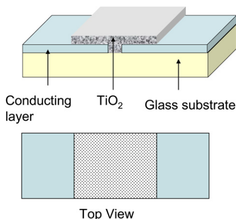
Fig. 1. Schematic diagram showing the geometry of the sample used for measurement of noise.
