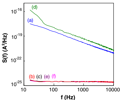
Fig. 3. Noise spectra of \text{TiO}_2 films under different conditions: (a) in \text{N}_2 (relative humidity 70%), (b) preheated sample in vacuum; (c) in dry nitrogen (preheated in vacuum at 90^\circ\text{C} for 5 min); (d) preheated in dry nitrogen after introduction of a trace amount of iodine; (e) dye coated film in dry nitrogen; and (f) dye coated film in dry nitrogen after introduction of iodine.
