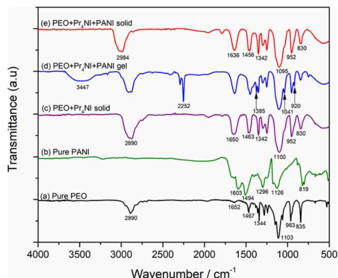
Fig. 6. FTIR spectra of (a) Pure PEO, (b) Pure PANI, (c) PEO + Pr_4NI solid electrolyte, (d) PEO + Pr_4NI + 1.5 wt% PANI gel electrolyte prior to vacuum drying and (e) PEO + Pr_4NI + 1.5 wt% PANI solid electrolyte in the region 500\text{--}4000\text{ cm}^{-1} .
