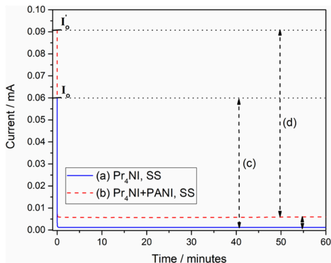
Fig. 4. Current vs time plots for solid polymer electrolyte samples obtained by DC polarization test with stainless-steel blocking electrodes. The values of the initial ( t = 0 ) currents are 0.06 mA for the PEO:Pr 4 NI electrolyte and 0.09 mA for the PEO:Pr 4 NI:PANI (1.5 wt%) electrolyte. The vertical distances (c) and (d) represent ionic conductivity parts for the two electrolytes.
