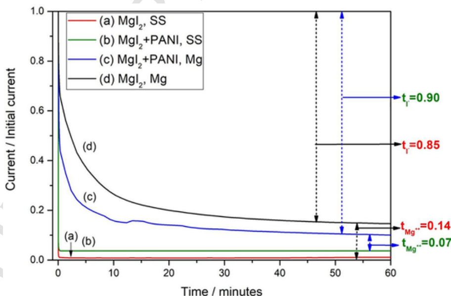
Fig. 5. Current/initial current vs time plots for PEO: \text{MgI}_2 solid electrolyte samples with and without PANI obtained by DC polarization test with Mg non-blocking electrodes and stainless-steel (SS) blocking electrodes.
