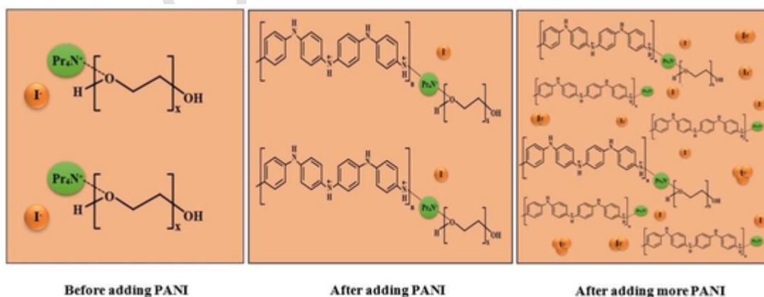
Fig. 8. Schematic diagram of the \text{PEO}:\text{Pr}_4\text{NI}:\text{PANI} solid polymer electrolyte showing the “cation trapping effect” due to interactions between \text{Pr}_4\text{N}^+ cations and PANI/PEO polymers allowing more iodide ions to be available for iodide ion conduction.
