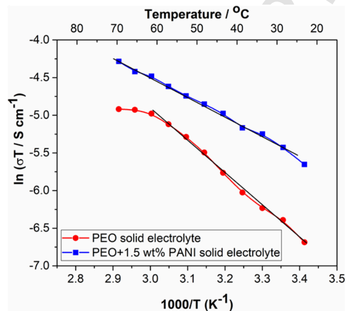
Fig. 2. \ln(\sigma T) vs 1000/T plots for PANI free PEO based solid polymer electrolyte and 1.5 wt% PANI added PEO based solid polymer electrolyte.
