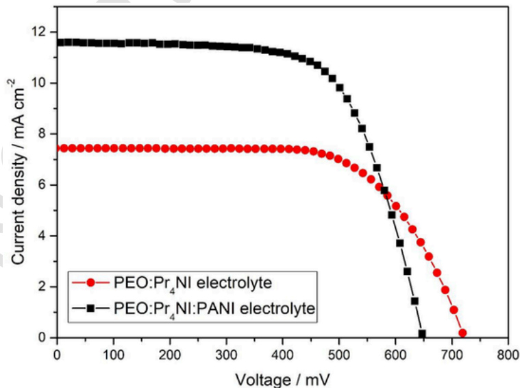
Fig. 9. Photocurrent density-voltage curves for DSSCs based on PEO + Pr_4NI (circles) and PEO + Pr_4NI + 1.5 wt% PANI (squares) solid polymer electrolytes.
