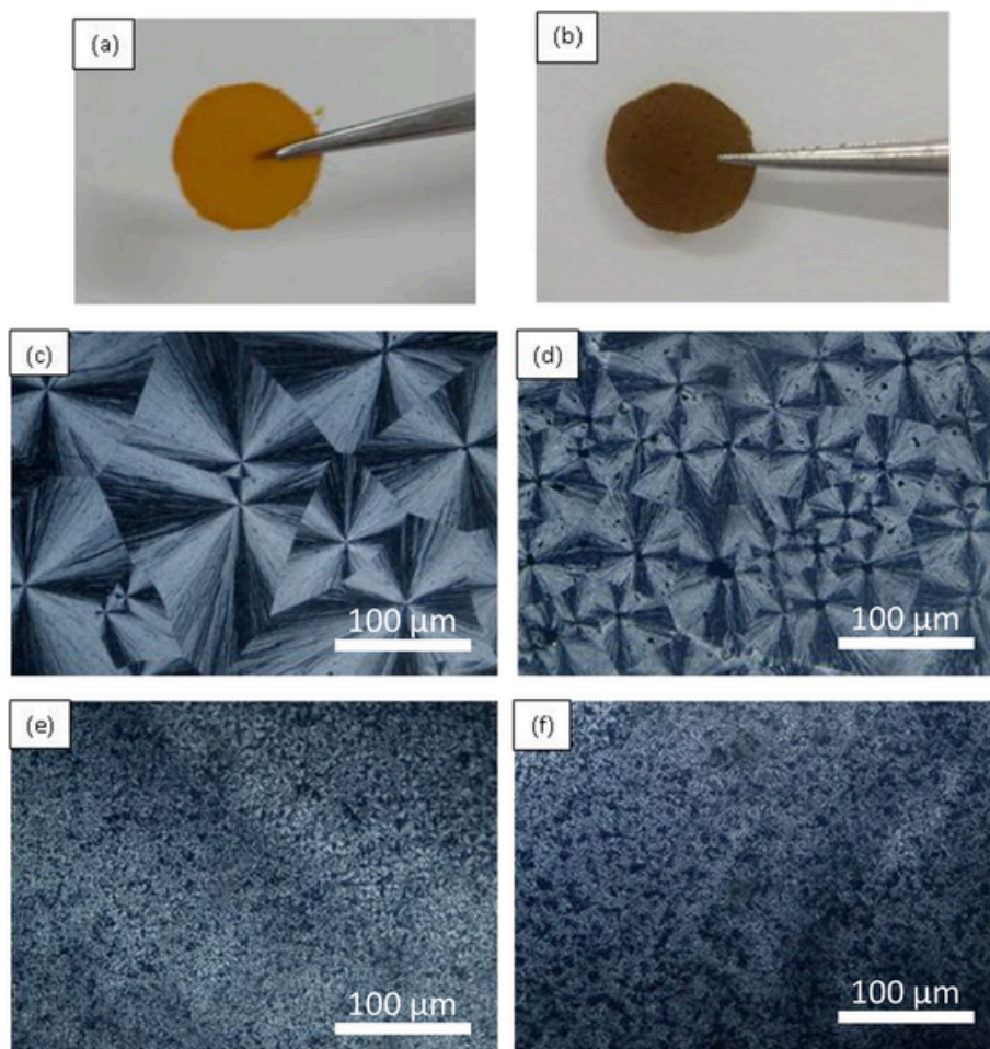
Fig. 3. Polarizing microscopy photographs of PEO based free standing solid electrolyte film, (a) without PANI additive, (b) with PANI additive. Cross-polarized optical micrographs of (c) pure PEO, (d) PEO/PANI mixed polymer film, (e) PEO/Pr 4 NI (EO:Pr 4 NI molar = 12:1) polymer electrolyte film without PANI additive and (f) PEO/Pr 4 NI (EO:Pr 4 NI molar = 12:1) polymer electrolyte film containing 1.5 wt% PANI. Same x100 magnification was used for all four images.
