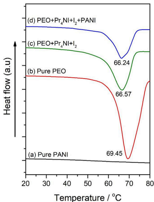
Fig. 7. DSC spectra of (a) pure PANI, (b) pure PEO, (c) PEO with optimum \text{Pr}_4\text{NI} salt and \text{I}_2 and (d) \text{PEO} + \text{Pr}_4\text{NI} + \text{I}_2 + 1.5 \text{ wt\% PANI} solid polymer electrolytes in the region 20^\circ\text{C} to 80^\circ\text{C} .
