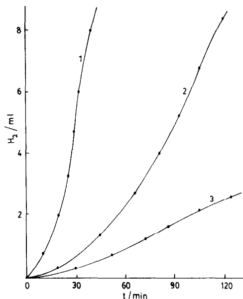
Fig. 1. Photogeneration of hydrogen from aqueous solutions of (1) 8.7 M ethanol, (2) 4.3 M ethanol and (3) 6.6 M acetic acid containing 0.2 M \text{H}_2\text{M} \text{H}_2\text{SO}_4 and 0.04 M \text{CuSO}_4 .
