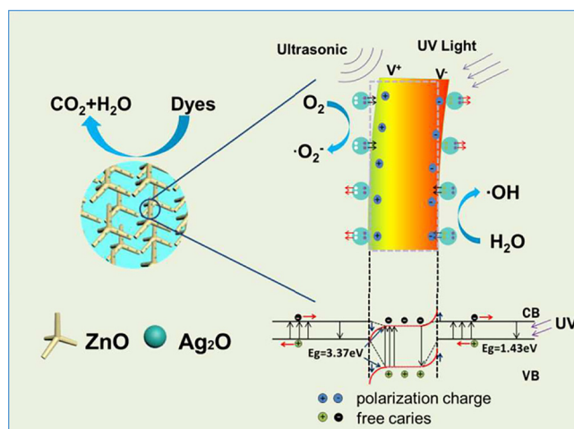
Fig. 8. Schematic illustration showing the working mechanism for the piezo-photocatalytic process of \text{Ag}_2\text{O}/\text{T-ZnO} nanostructures under ultrasonic and UV exposure. Reproduced with permission [120].
